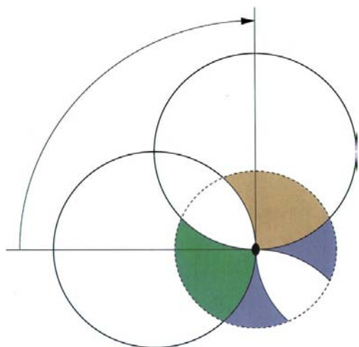
Figure 19 The fractional completeness is higher than the fraction of the required rotation range; 90^\circ rotation out of 180^\circ gives about 65% of unique data.
